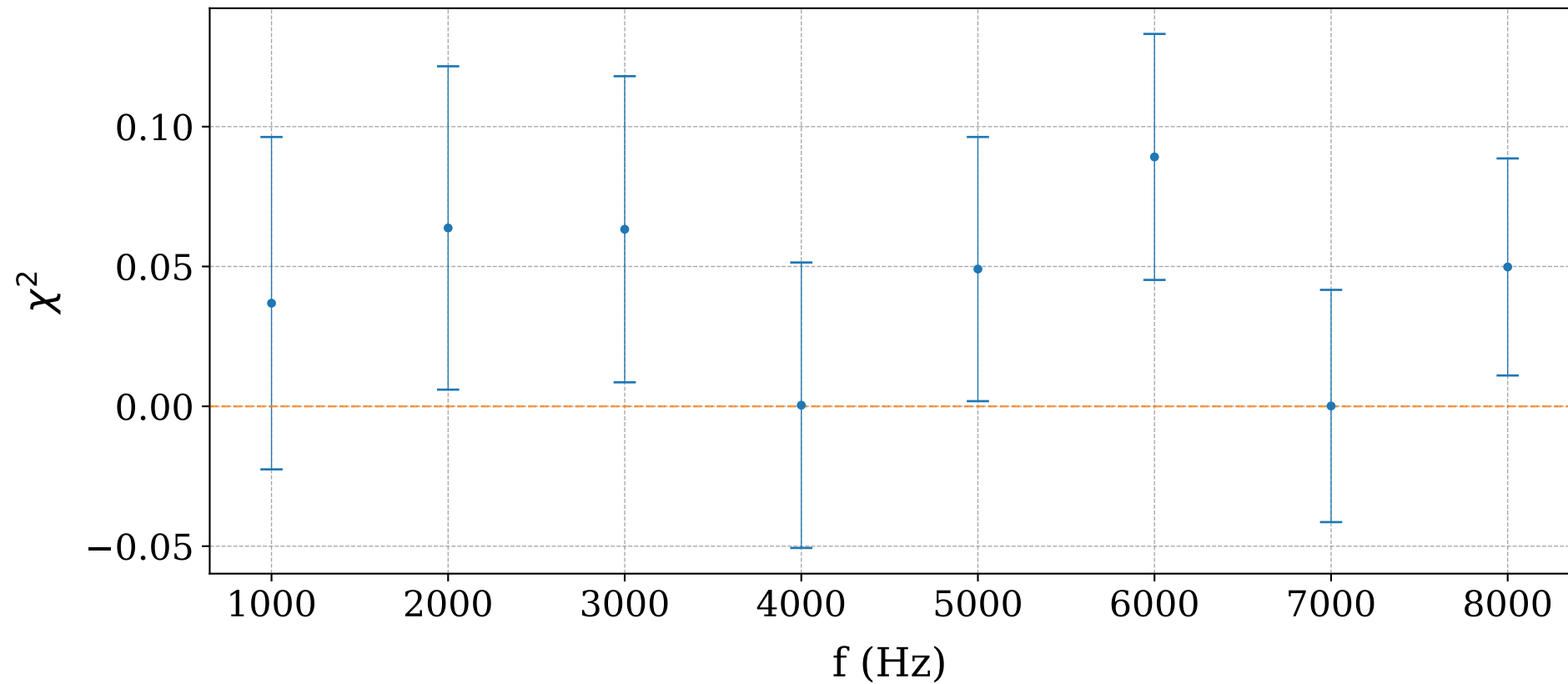
Fit Lineare A, \chi^2
